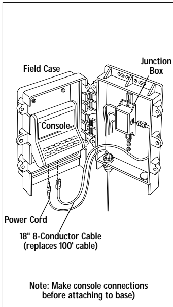
EZ-MOUNT WEATHER STATION
